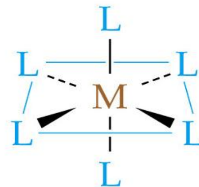
Octahedral
