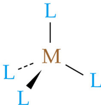
Tetrahedral
